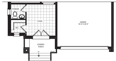
ELEVATION C GROUND FLOOR
