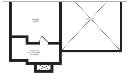
ELEVATION B BASEMENT
