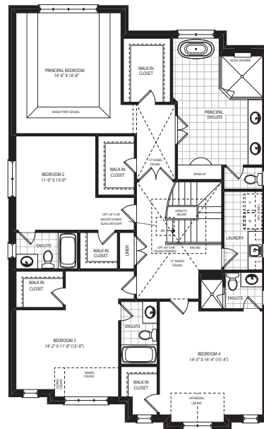
ELEVATION A SECOND FLOOR
