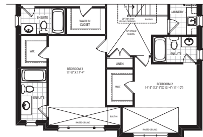
ELEVATION C SECOND FLOOR
